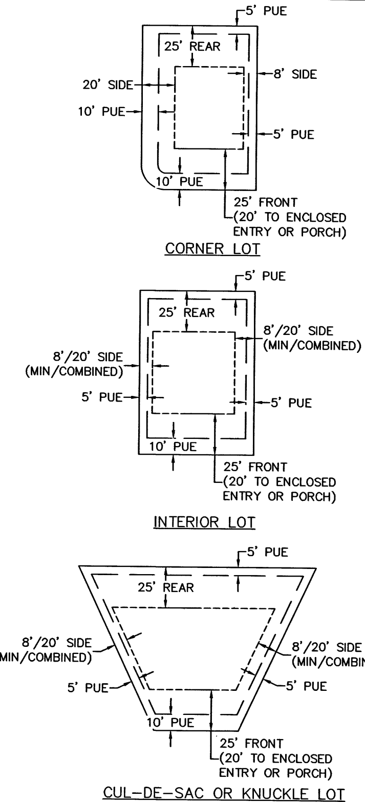
TYPICAL SETBACK & P.U.E. DETAILS
